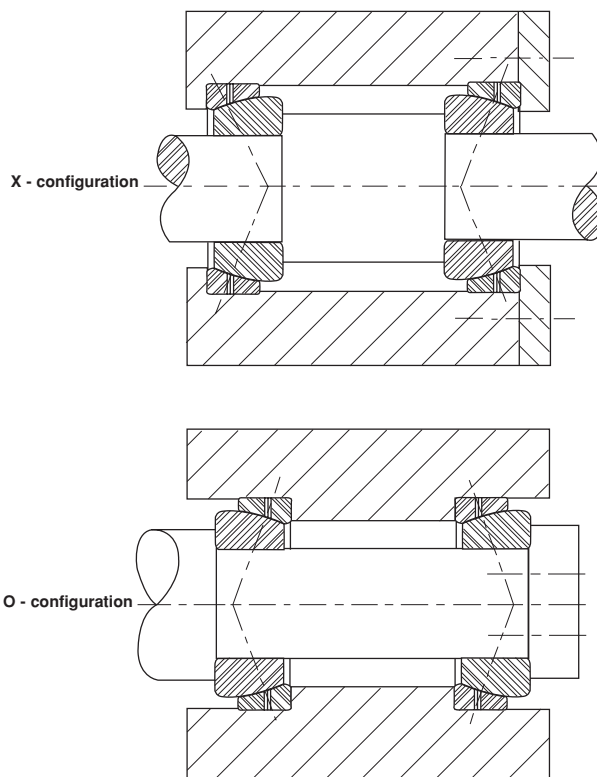
Figure 10: Bearing Arrangement
