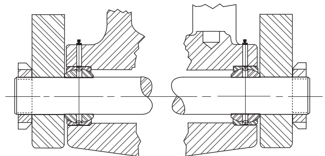
Steering Axle
